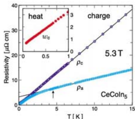
Fig. 3. Anisotropic quantum criticality. Electrical resistivity at the QCP (at H = 5.3 , T \cong H_c ) for in-plane ( \rho_a ) and inter-plane ( \rho_c ) current directions. \rho_c(T) remains linear over a 100-fold increase in magnitude. By contrast, \rho_a is linear only above a characteristic fluctuation temperature T_{SF} \cong 4 K (arrow) (18). (Inset) Thermal resistivity ( w_c = L_0 T / \kappa_c ) at the QCP, for inter-plane transport. w_c is perfectly linear down to the lowest temperature.
